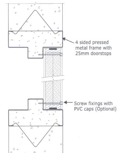
Wall panel with pressed metal door frame
