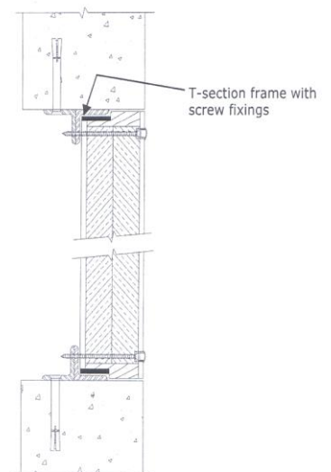
Wall panel with T-Section frame
